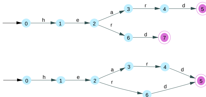
Figure 3. Example Algorithm Semi-Incremental: Adding word ‘herd’
