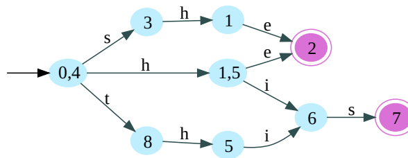
Figure 6. Merged automaton
